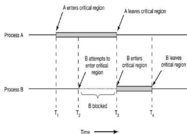
Figure 49: Mutual Exclusion Using Critical Regions
