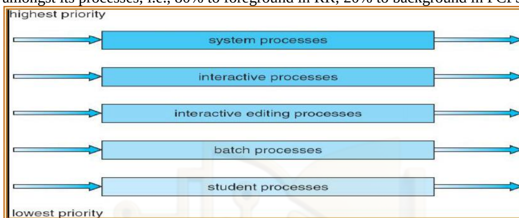
Figure 47: Multi Level Queue Scheduling
