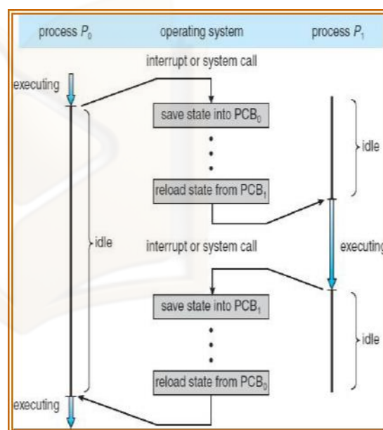
Figure 29: CPU switching between processes
