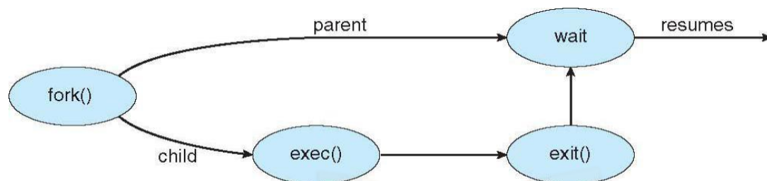
Figure 32: Fork () Process
