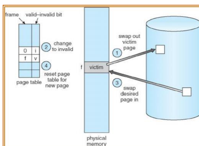
Figure 86: Page replacement
