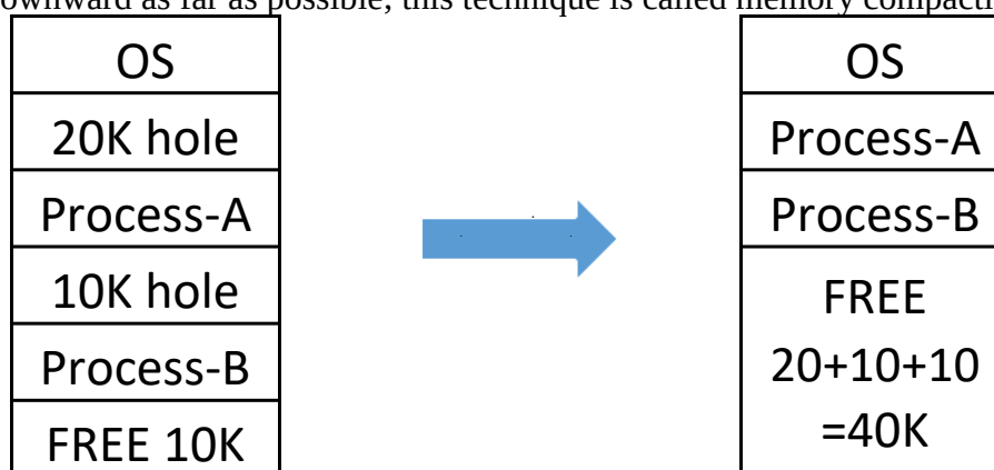
Figure 69: Compaction
