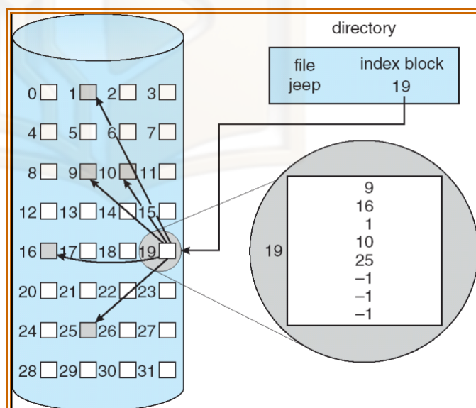
Figure 126: Index Allocation
