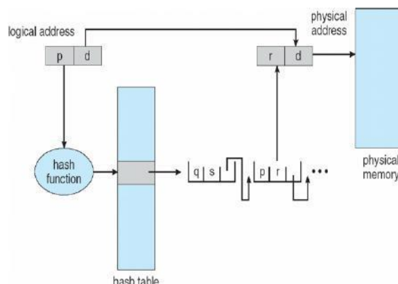
Figure 77: Hashed Page Tables
