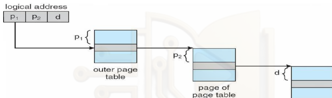
Fig: Address translation scheme
