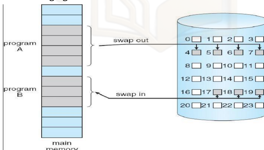
Figure 83: Transfer of a paged memory to continuous disk space
