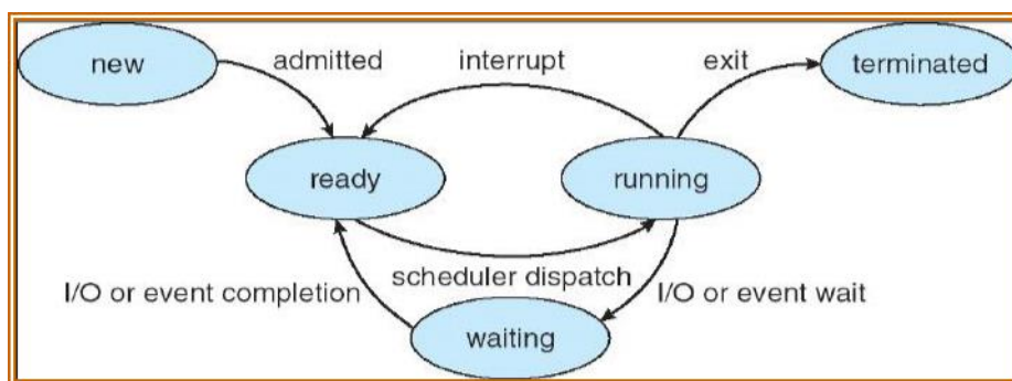
Figure 26: Diagram for Process State
