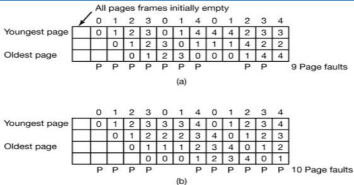
Figure 90: Belady's anomaly. (a) FIFO with three page frames. (b) FIFO with four page frames. The P's show which page references cause page faults.
