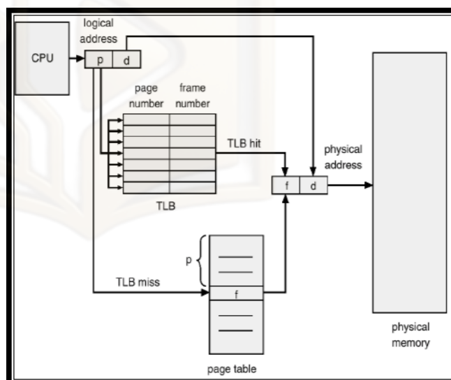
Figure 76: Paging Hardware with TLB
