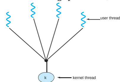
Figure 41: Many to one model.
