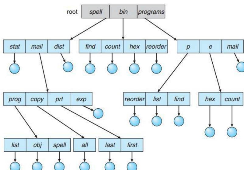
Figure 119: Tree structured directories
