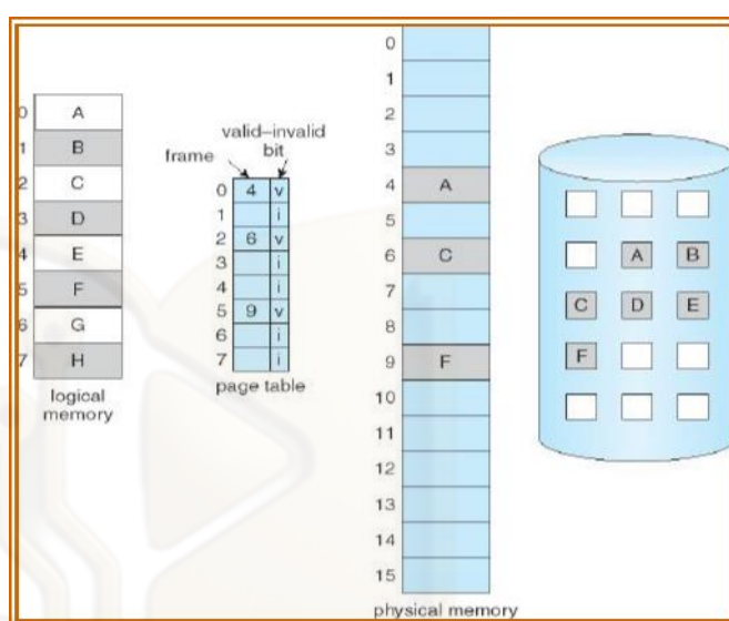
Figure 84: The Picture When All Pages Are Not In Memory
