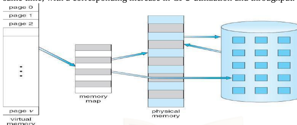
Figure 82: Diagram showing virtual memory that is larger than physical memory.
