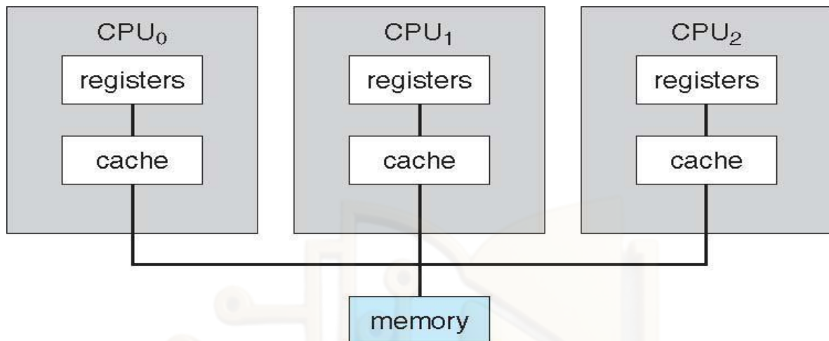
Figure 4: Symmetric multiprocessor architecture
