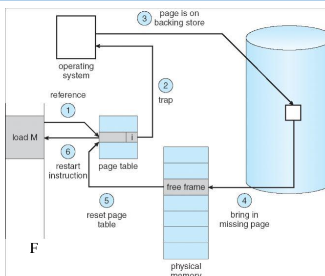
Figure 85: The Picture When All Pages Are Not In Memory
