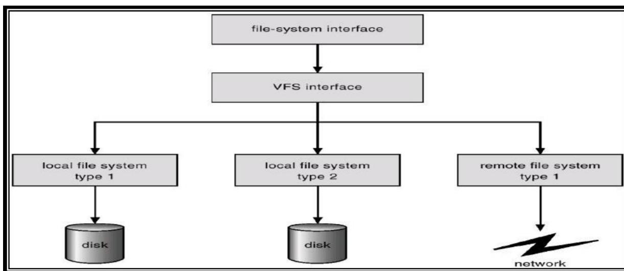
Figure 122: Systematic view of virtual file system
