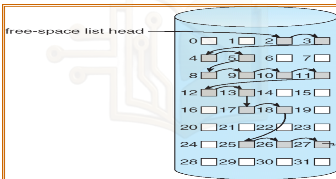
Figure 129: Linked List scheme
