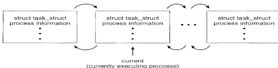
Figure 28: Active process in Linux
