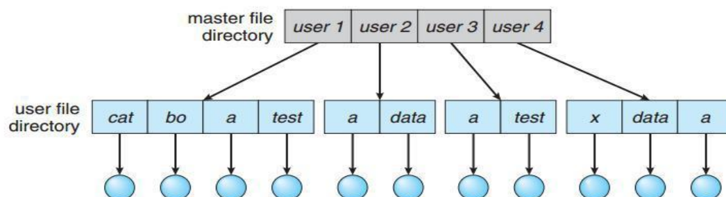
Figure 118: Two Level Directory
