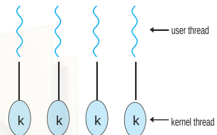
Figure 42: One to One Thread
