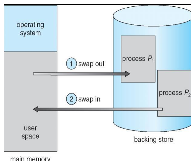
Figure 70: Swapping of two processes using a disk as a backing store
