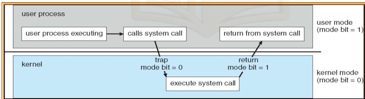
Figure 6: Transition from user mode to kernel mode
