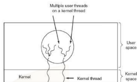
Figure 39: Hybrid Thread
