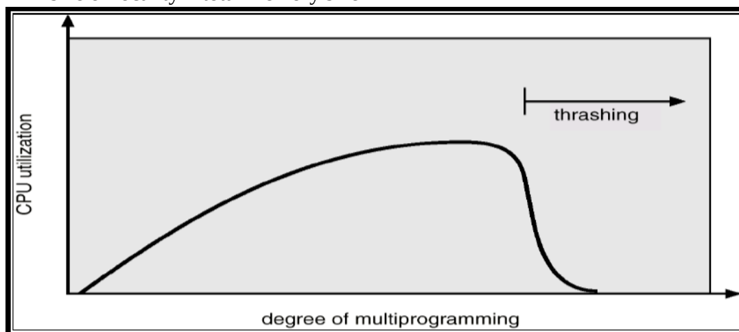
Figure 91: Thrashing
