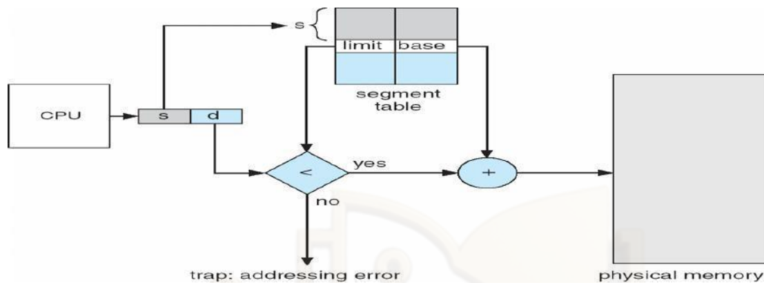
Figure 80: Segmentation hardware
