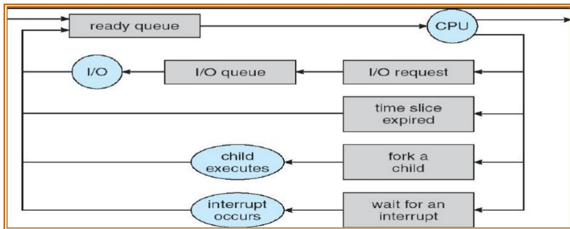
Figure 30: Queuing Diagram
