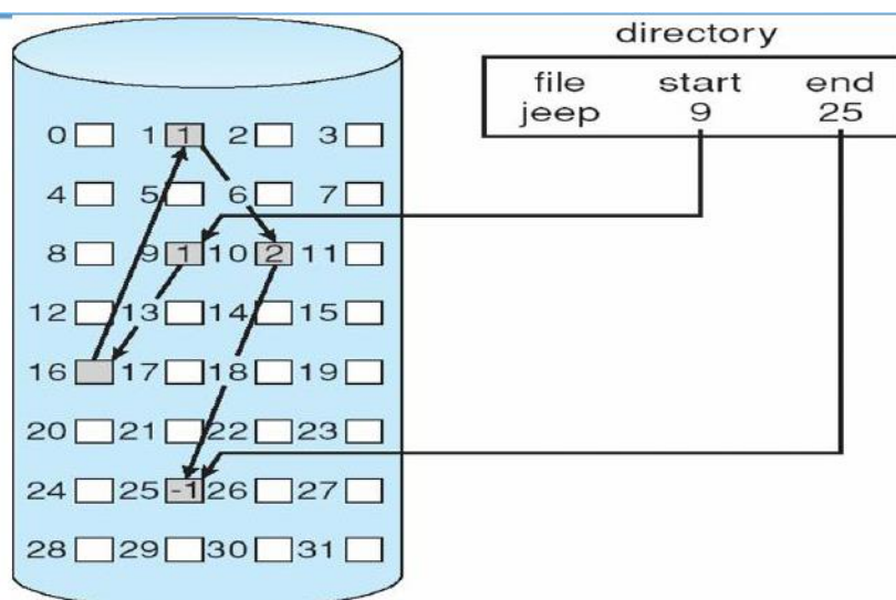
Figure 124: Linked Allocation
