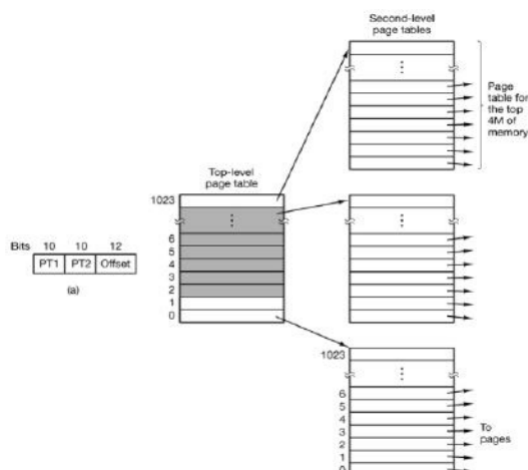
Figure 75: (a) A 32-bit address with two page table fields.
