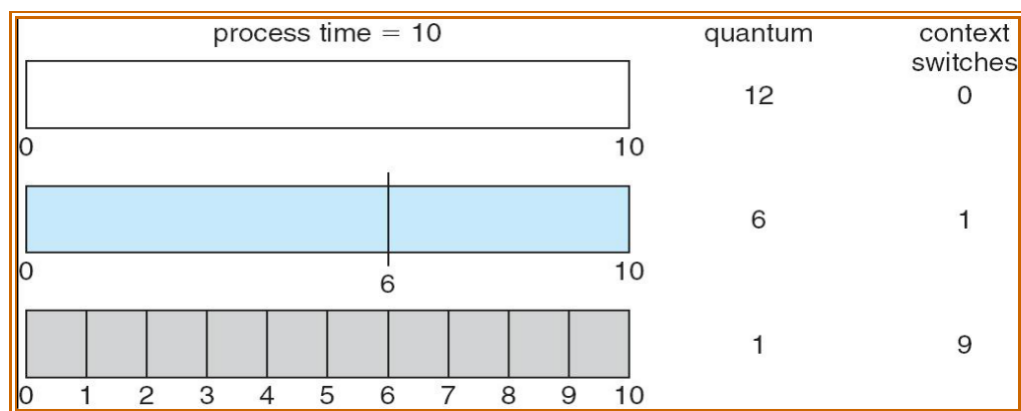
Figure 45: How a smaller time quantum increases context switches
