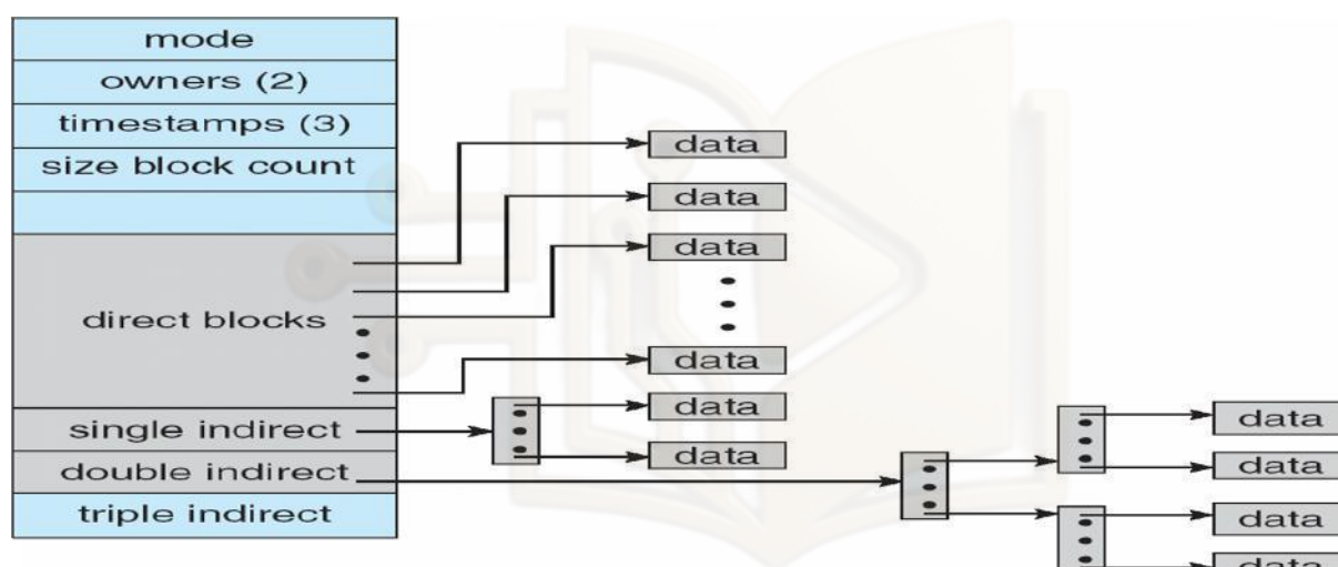
Figure 128: Combined Scheme: UNIX UFS
