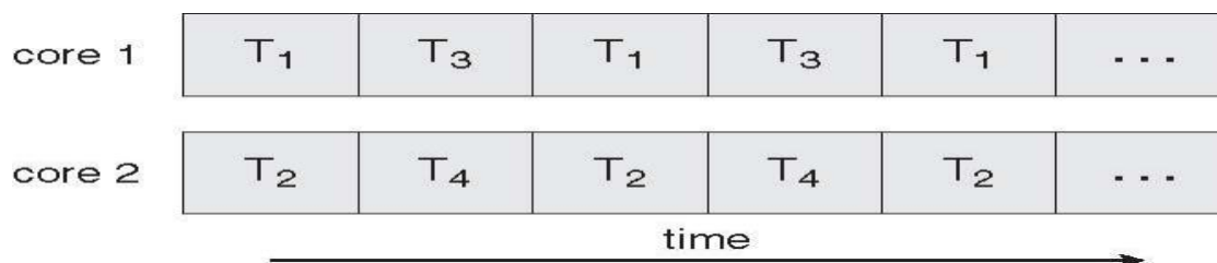
Figure 36: Parallel Execution on a Multi Core system
