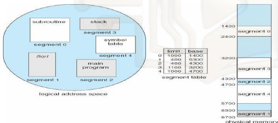
Figure 81: Example of Segmentation
