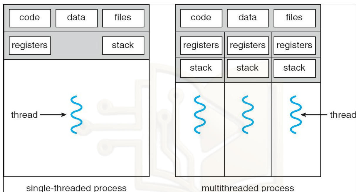
Figure 34: Single and multithreaded process.
