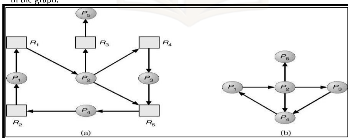
Figure 60: (a): Resource Allocation Graph Fig (b): Corresponding Wait for Graph
