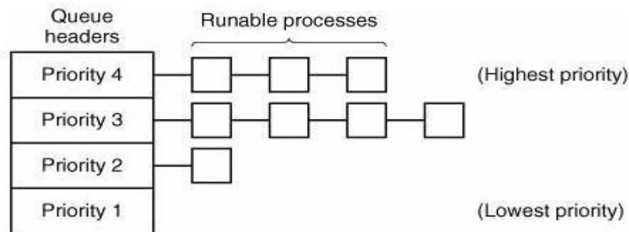
Figure 44: A scheduling algorithm with four Priority classes
