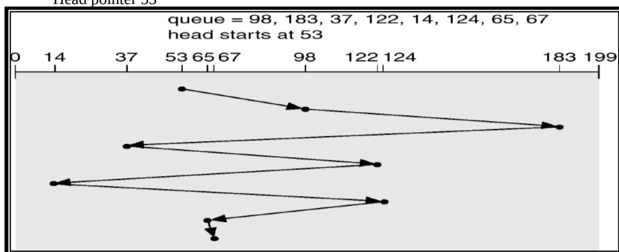
Figure 106: FIFO disk scheduling algorithm
