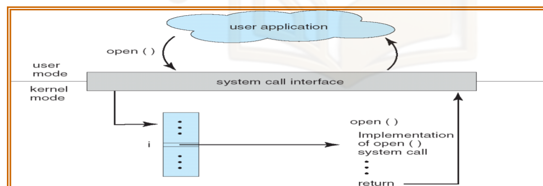
Figure 13: API, system call and OS relationship
