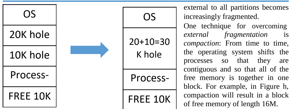
Figure 68: Coalescing
