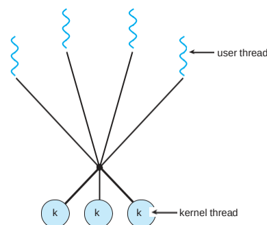
Figure 40: Many-to-Many Model
