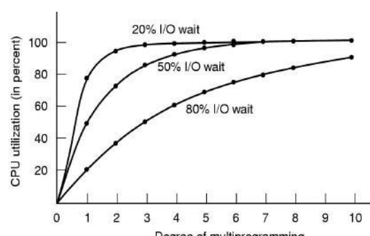
Fig: CPU utilization as a function of number of processes in memory
