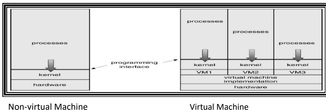
Figure 24: Virtual machines
