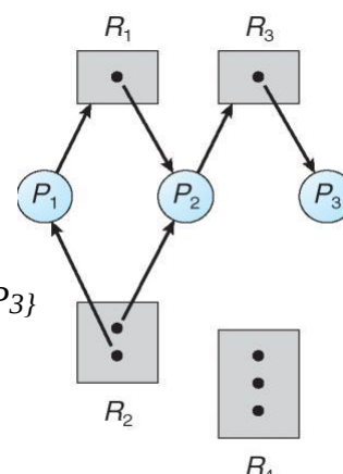
Fig: Resource allocation graph
