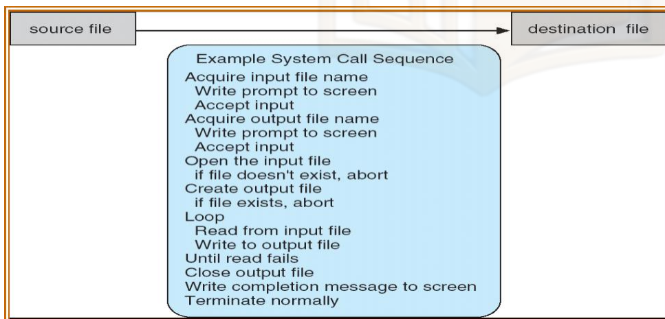
Figure 12: Example of system call
