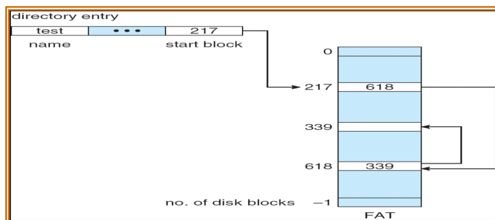
Figure 125: File Allocation Table
