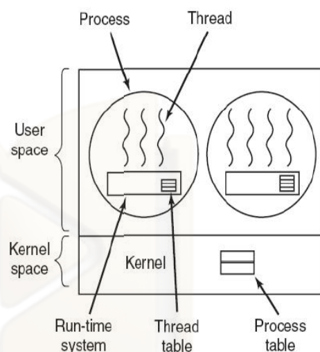
Figure 37: User Level Thread
