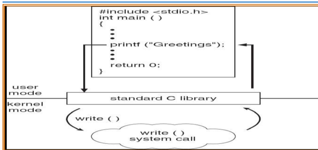
Figure 14: API, system call and OS relationship
