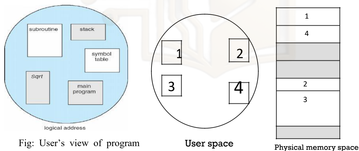
Figure 79: Logical view of segmentation
