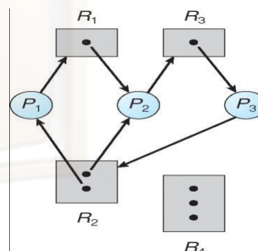
Figure 55: Resource Allocation Graph with Deadlock
