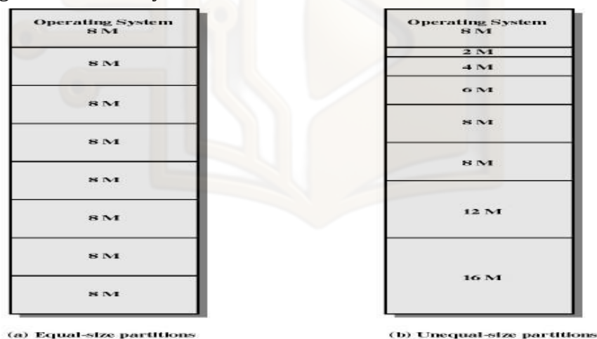
Figure 7.2 Example of Fixed Partitioning of a 64-Mbyte Memory
