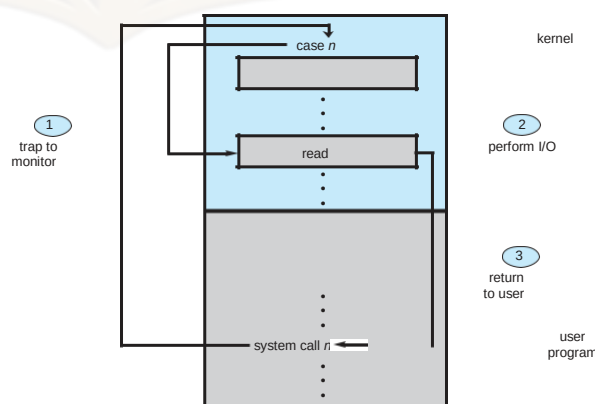
Figure 99: Use of a System Call to Perform I/O:
