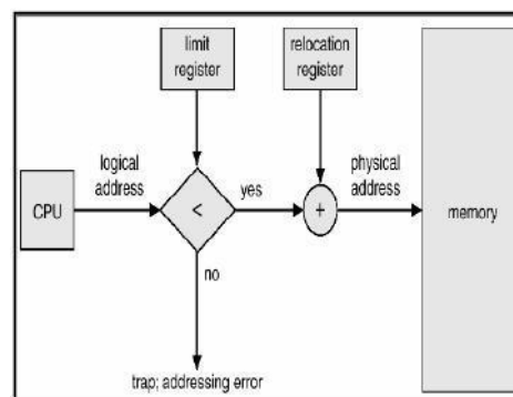
Figure 64: Memory protection using relocation register
