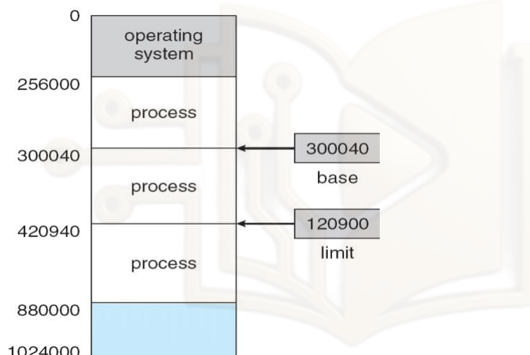
Figure 61: A base and limit register define a logical address space.
