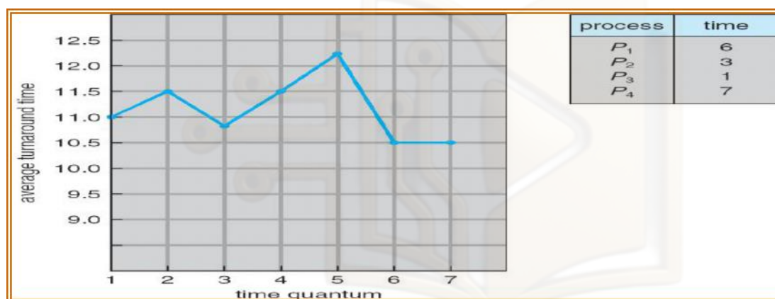
Figure 46: Turnaround time varies with quantum time
