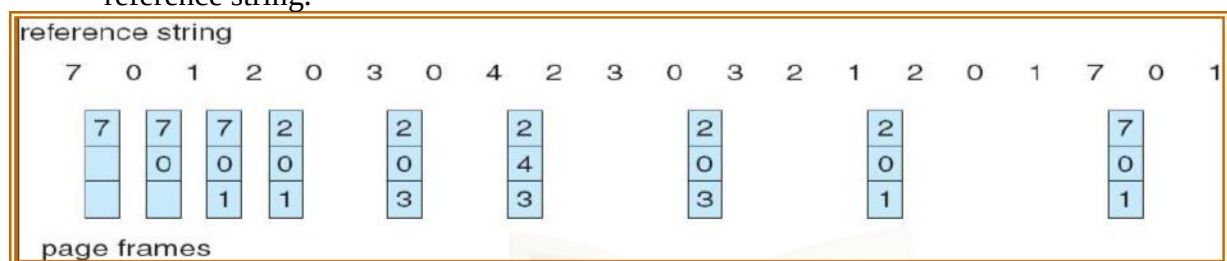
Figure 88: Optimal page replacement algorithm
