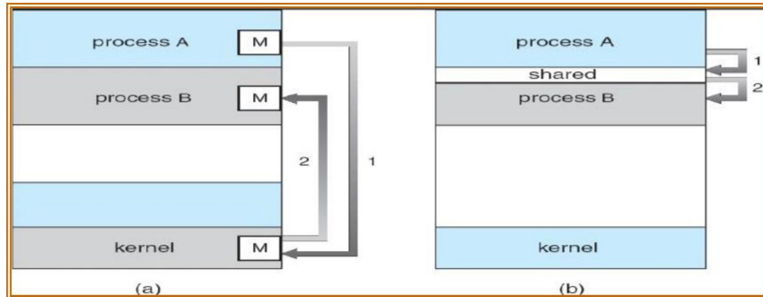
Figure 33: Communication Model (a) Message Passing (b) Shared Memory
