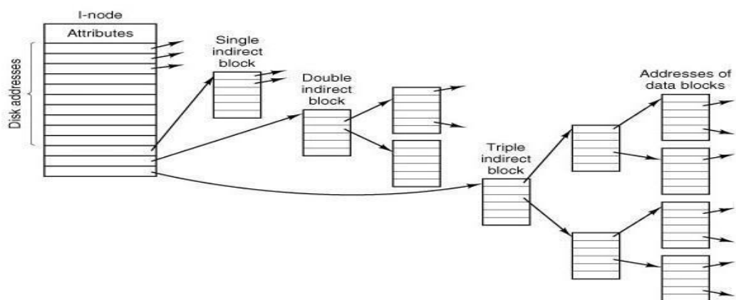
Figure 127: An i-node with three levels of indirect blocks
