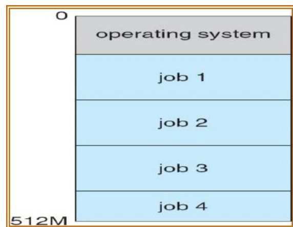
Figure 9: Memory layout for a multiprogramming system
