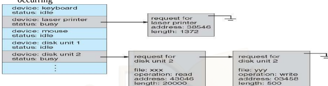
Figure 98: Device Status Table
