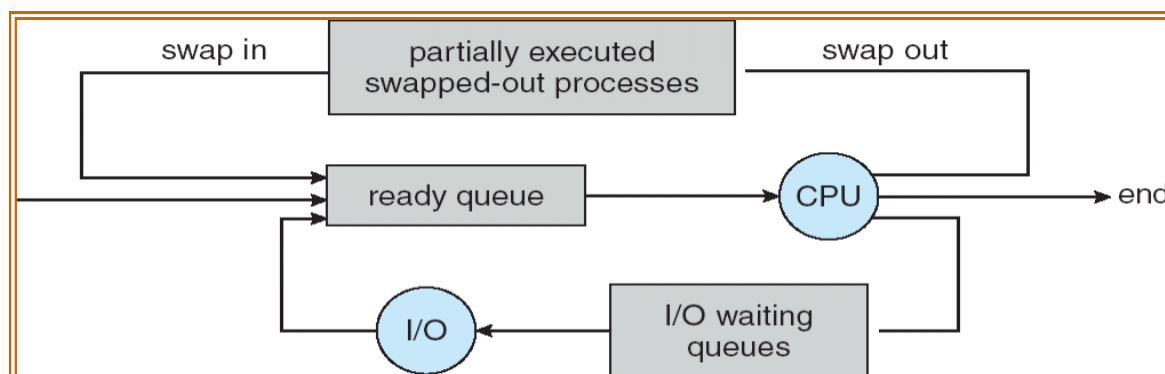
Figure 31: Queueing diagram with medium term scheduler
