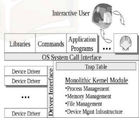
A monolithic kernel, such as Linux and other Unix systems.
