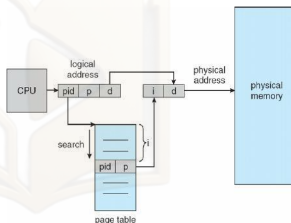
Figure 78: Inverted Page Table
