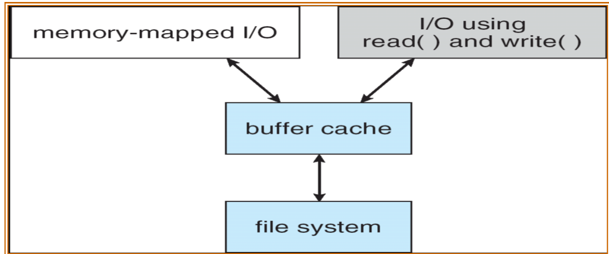
Figure 131: I/O using unified buffer
