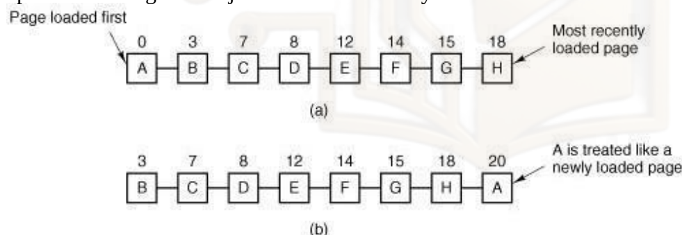
Fig: Operation of second chance. (a) Pages sorted in FIFO order. (b) Page list if a page fault occurs at time 20 and A has its R bit set. The numbers above the pages are their loading times.
