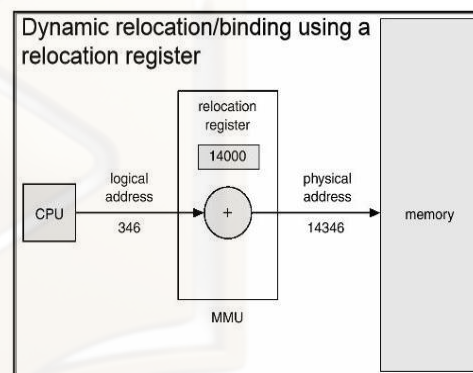
Figure 63: Dynamic relocation using relocation register
