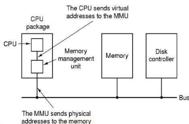
Figure 62: Memory management Unit
