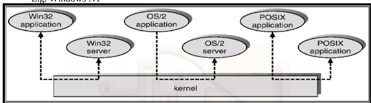
Figure 23: Client Server structure
