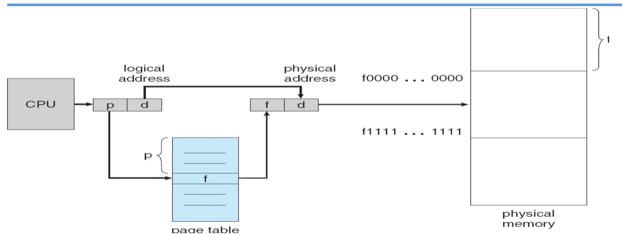
Figure 71: Paging Hardware
