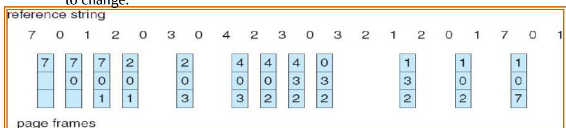
Figure 89: LRU page replacement algorithm
