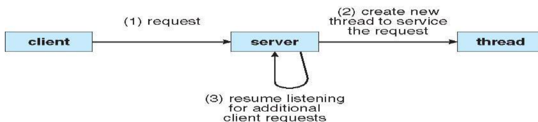
Figure 35: Multithreaded Server Architecture
