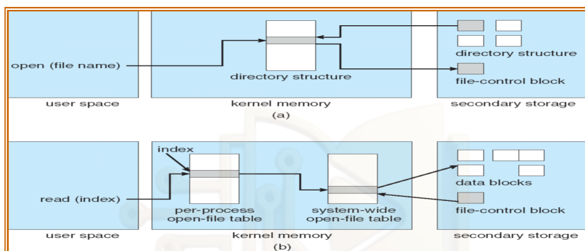
Figure 121: Opening and Reading a file (a) refers to opening a file (b) refers to reading a file
