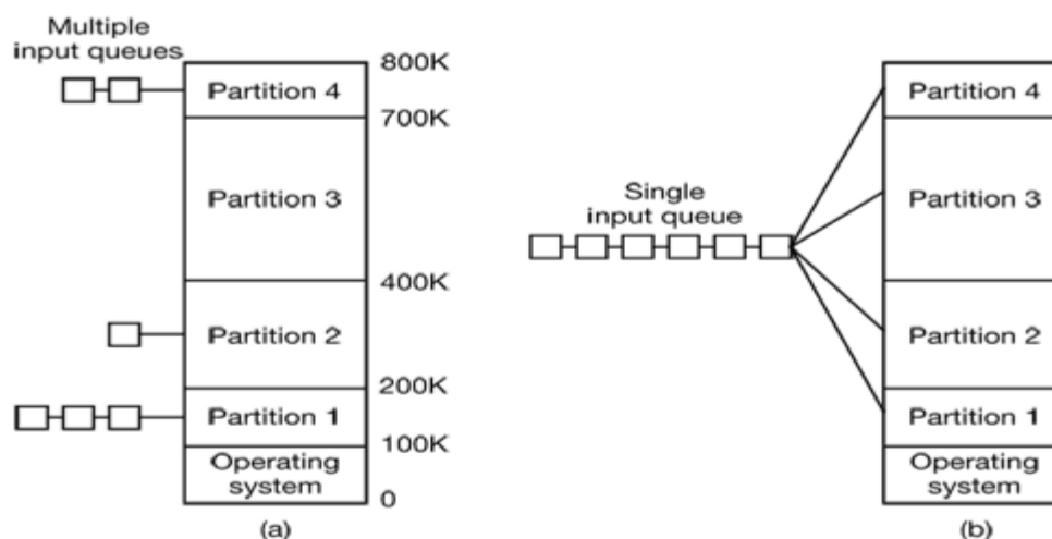
Figure 66: (a) Fixed memory partitions with separate input queues for each partition. (b) Fixed memory partitions with a single input queue
