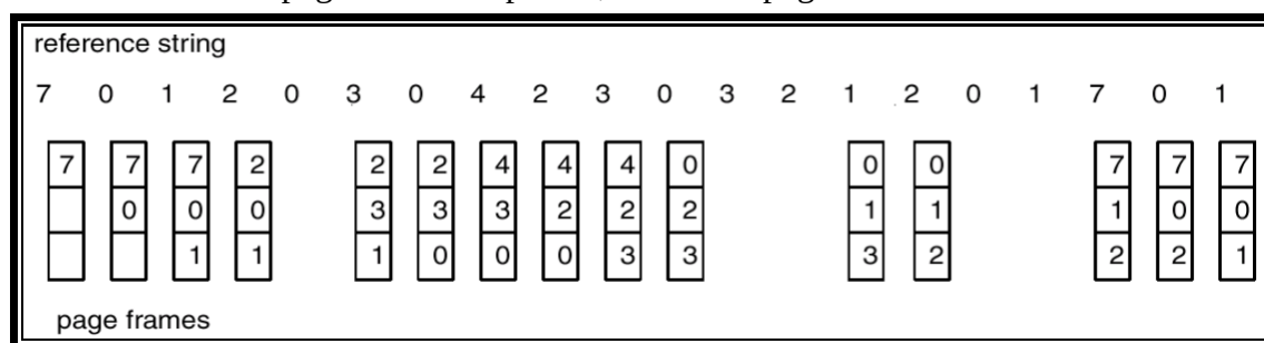
Figure 87: FIFO page replacement algorithm
