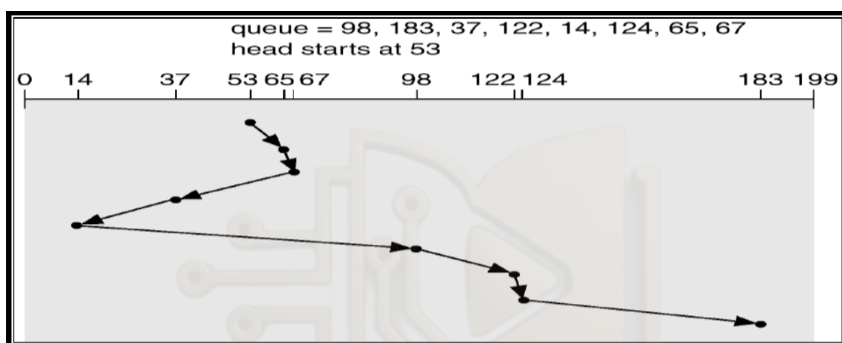
Figure 107: SSTF disk scheduling Algorithm
